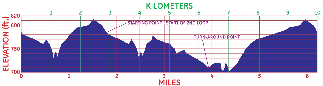
Course Elevation
